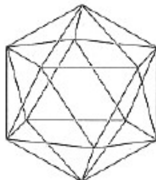
Icosahedron
