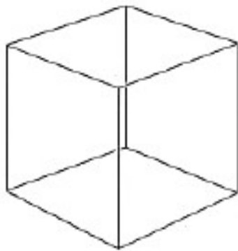
Cube
