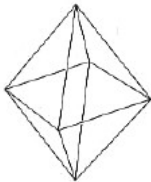
Octahedron
