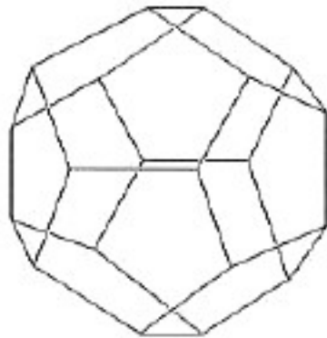
Dodecahedron
