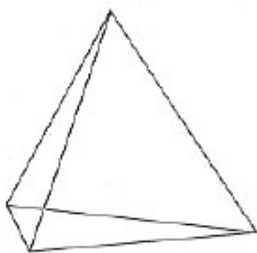
Tetrahedron
