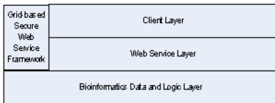
Figure 1 GSWSF layers.
