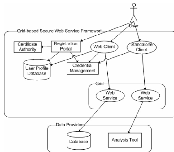
Figure 2. Component Diagram of GSWSF
